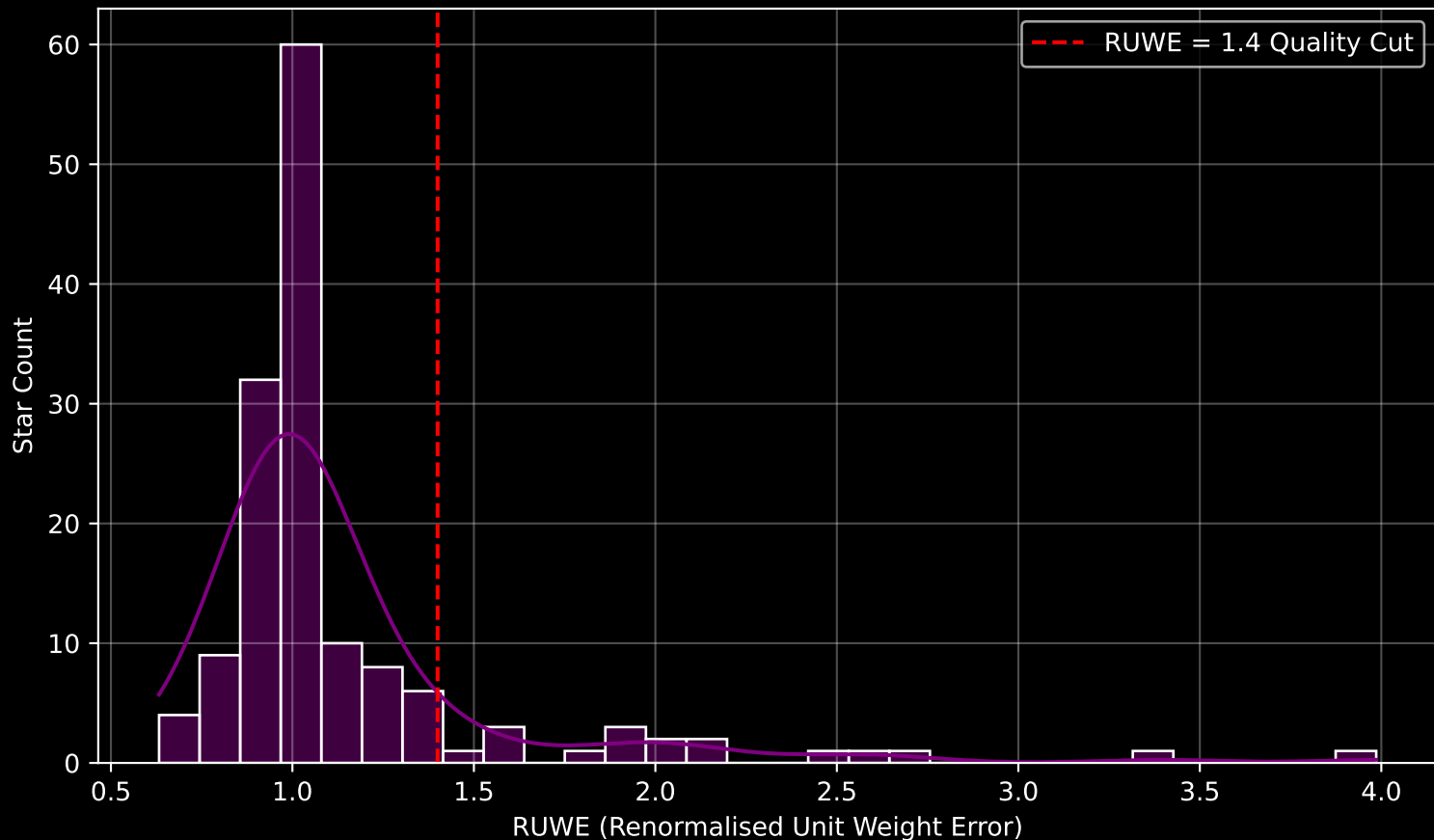
GAPOGEE DR17 Field [357-04-O] RUWE Distribution (n= 146)
