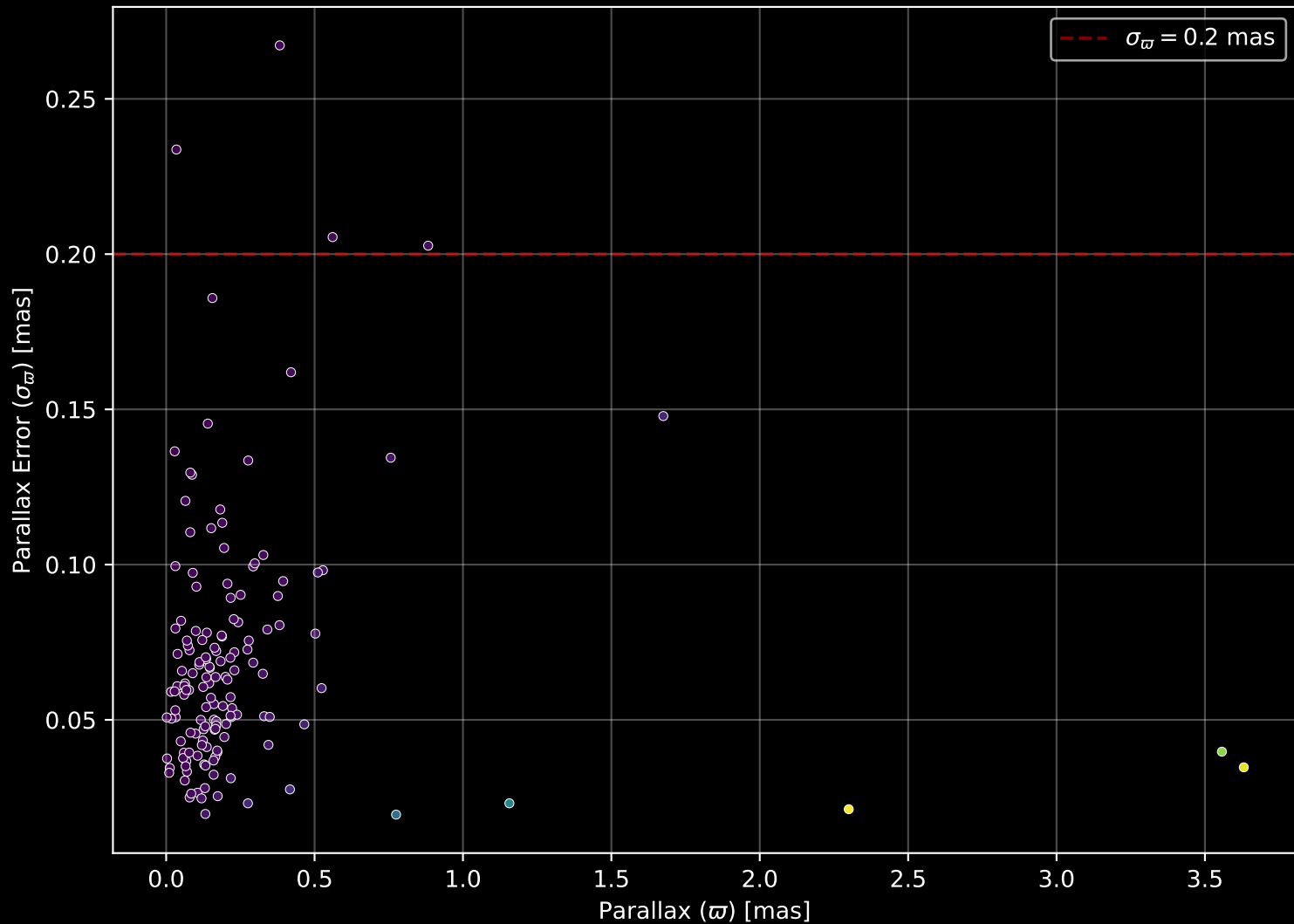
APOGEE DR17 Field: [357-04-O] Parallax Quality (n= 147)
