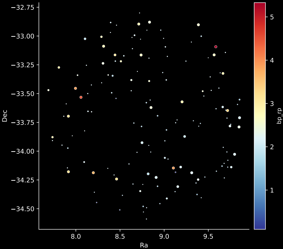
APOGEE DR17 Field: [357-04-O] Stars: 147
