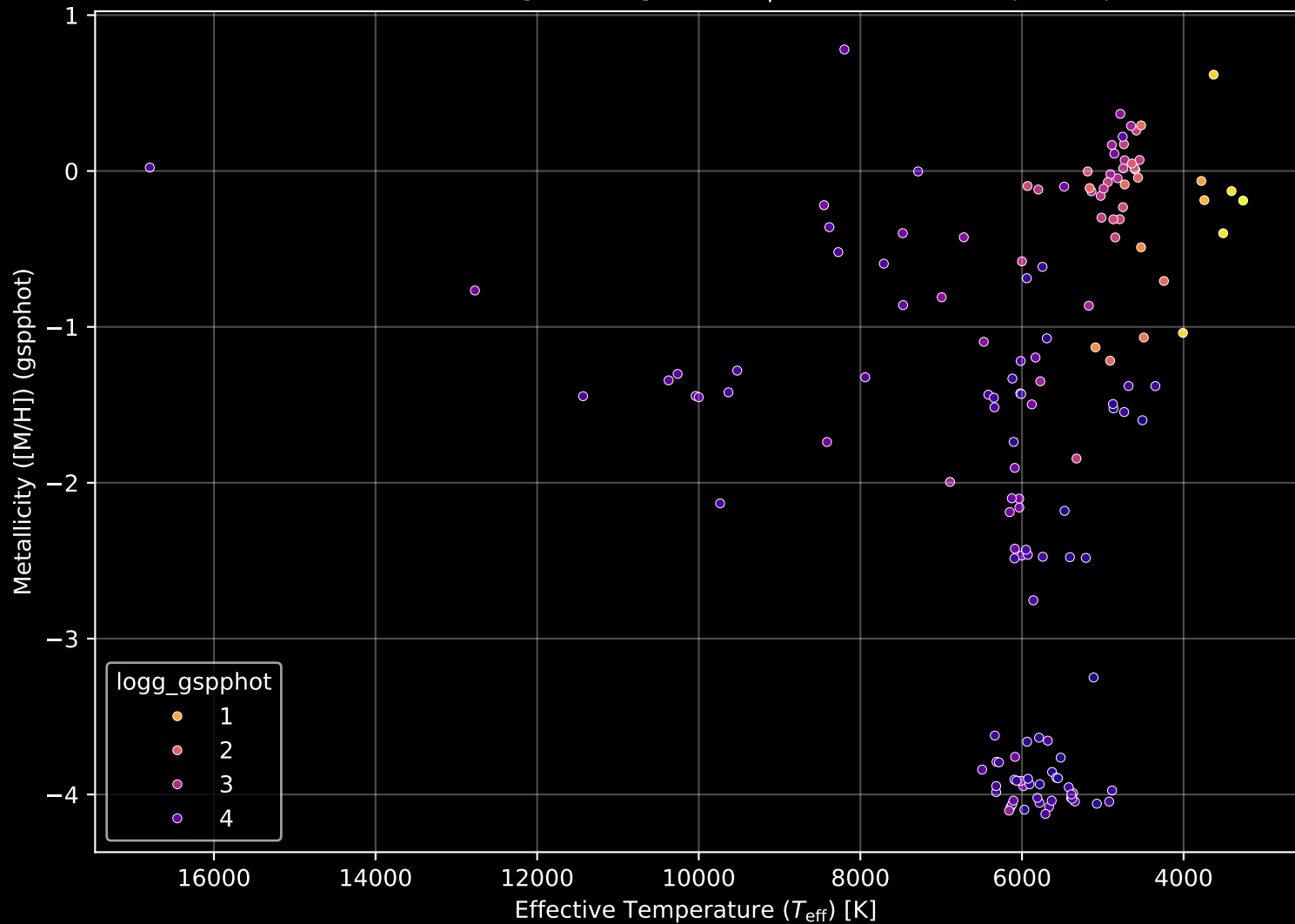
APOGEE DR17 Field: [357-04-O] Stellar Population Parameters (n= 147)
