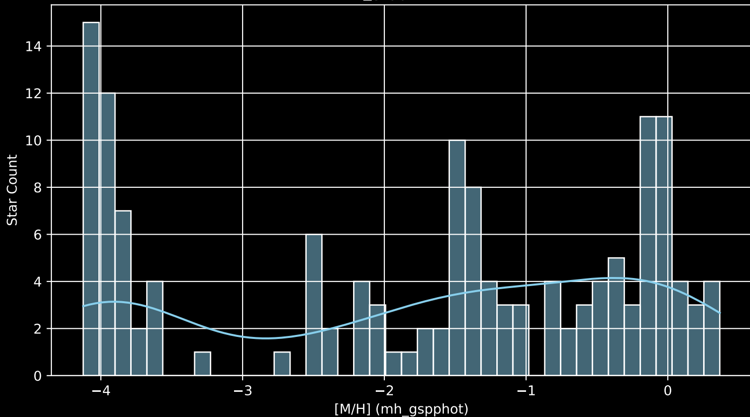
APOGEE DR17 Field: [357-04-O [M/H] (mh_gspphot) (n= 145)
