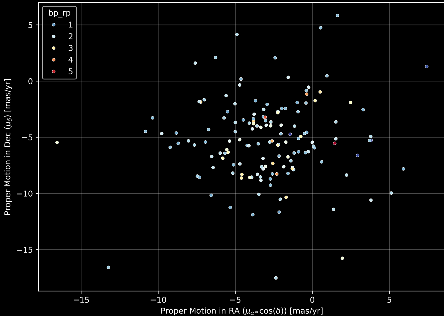
APOGEE DR17 Field: [357-04-O] Proper Motion Diagram (n= 147)
