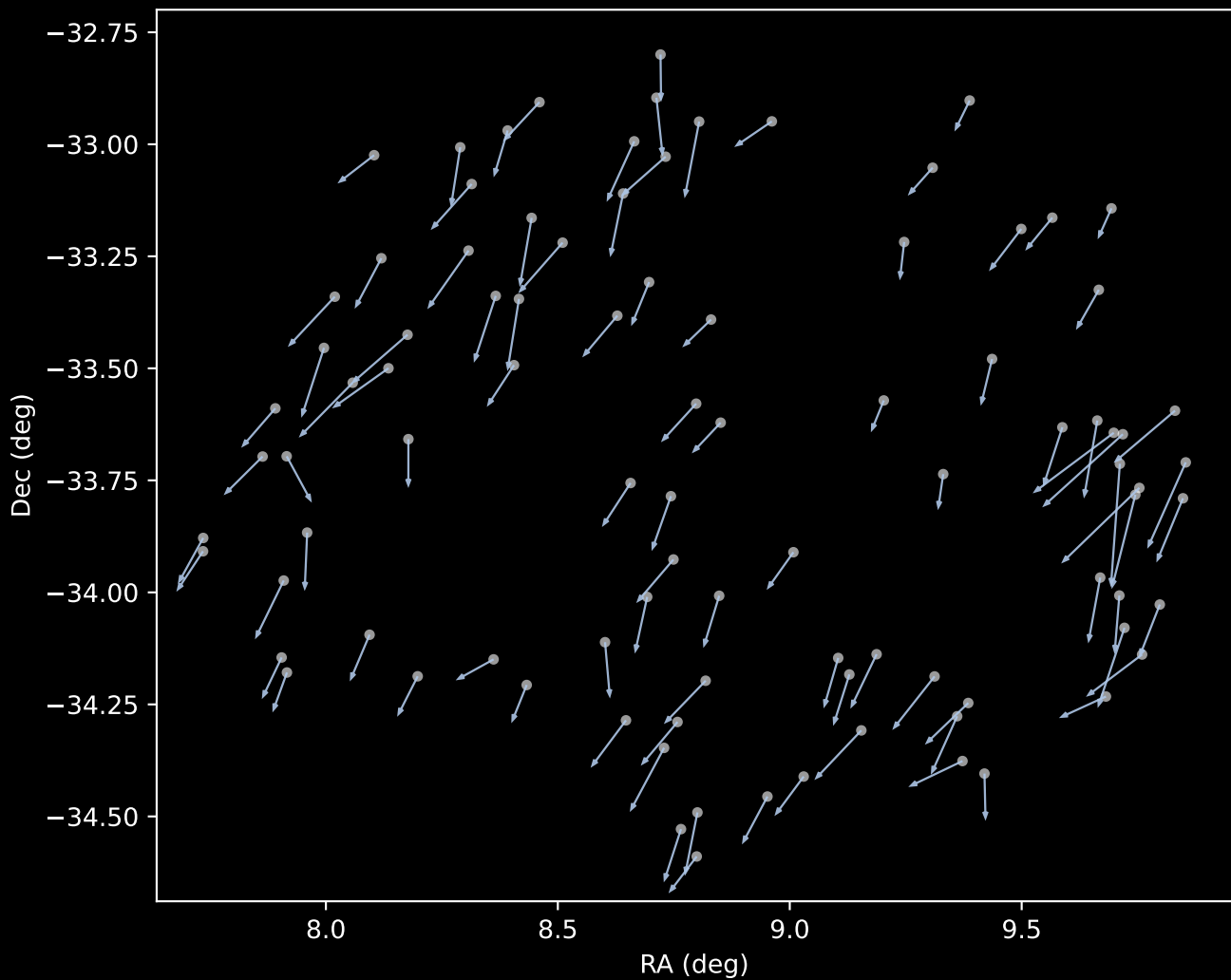
APOGEE DR17 Cluster 1 Proper Motion Vectors (n=94)
