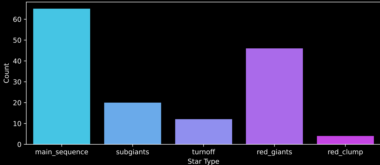
APOGEE DR17 Field: [357-04-O] Count plot of Star Type
